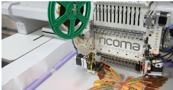
SEQUIN DEVICE
